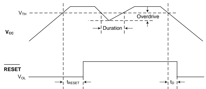
Figure 3. V_{CC} Transient
