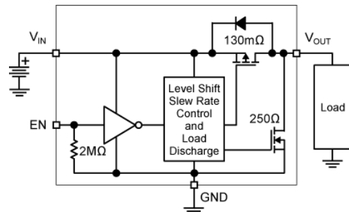
MIC94091 (ultra fast turn on with auto-discharge) MIC94093 ( 790\mu\text{s} soft-start with auto-discharge) MIC94095 ( 120\mu\text{s} soft-start with auto-discharge)
