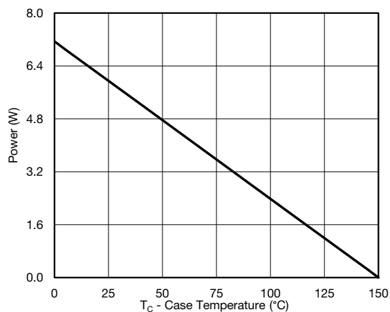
Power, Junction-to-Foot
