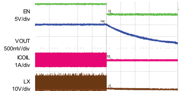
Fig. 14 - Shut-Down, I_{OUT} = 0 \text{ A} Time = 200 \text{ms/div}
