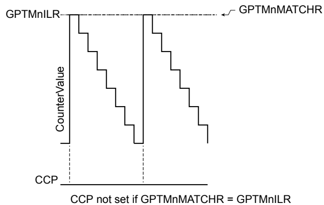
Figure 13-6. CCP Output, GPTMTnMATCHHR = GPTMTnILR
