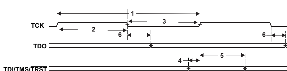
Figure 6-89. JTAG Test-Port Timing
