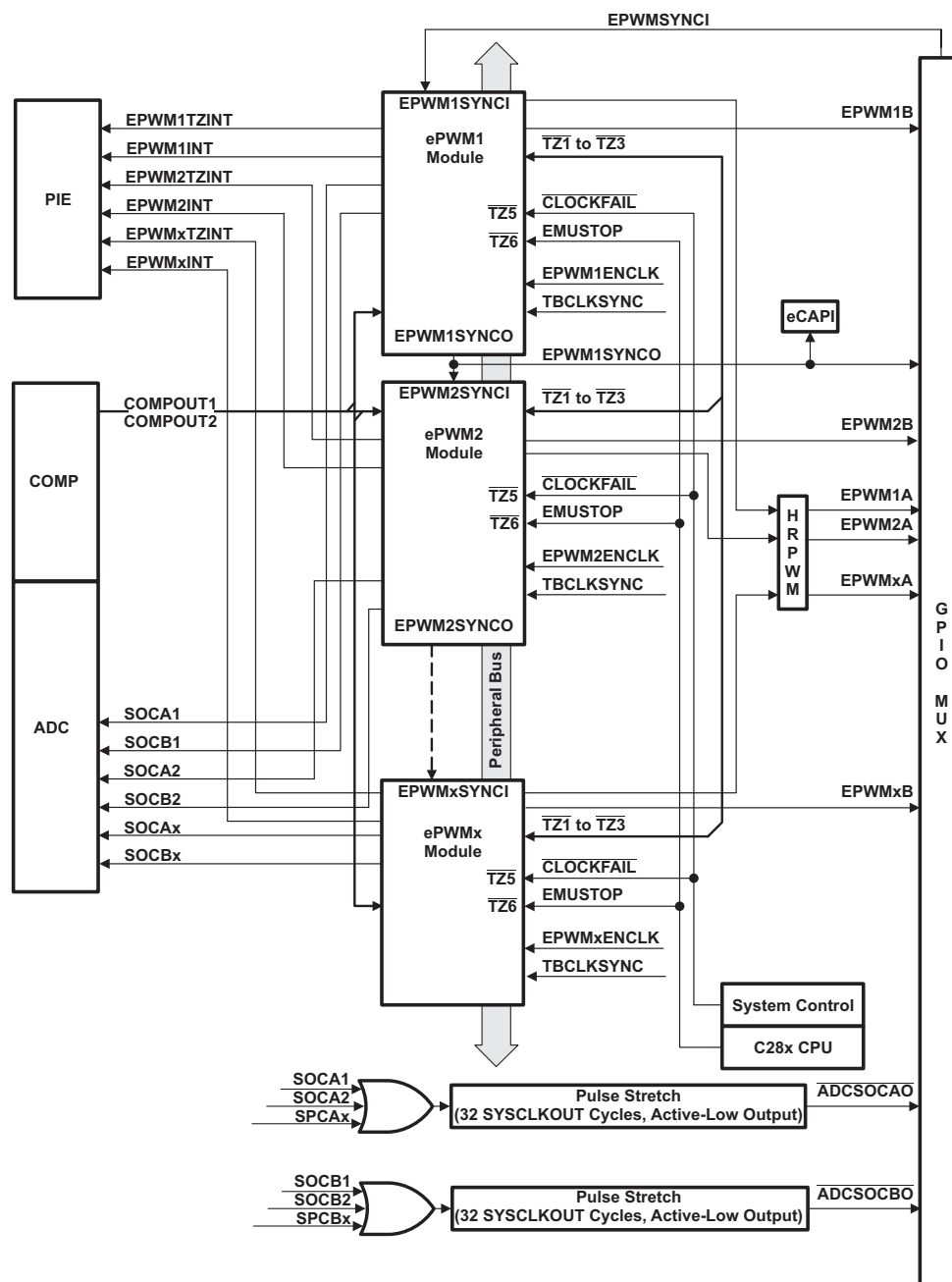
Figure 4-8. ePWM
