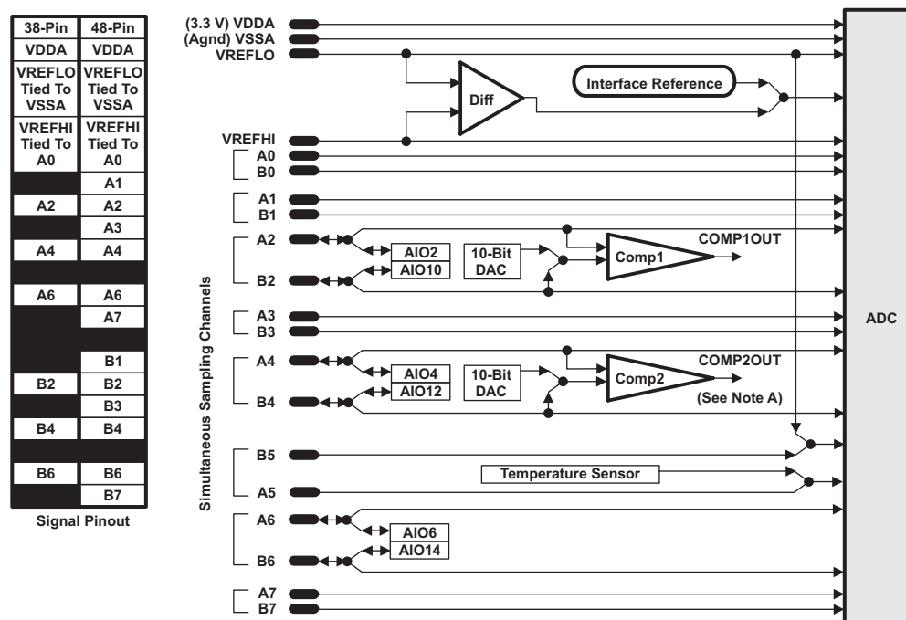
Figure 4-1. Analog Pin Configurations
