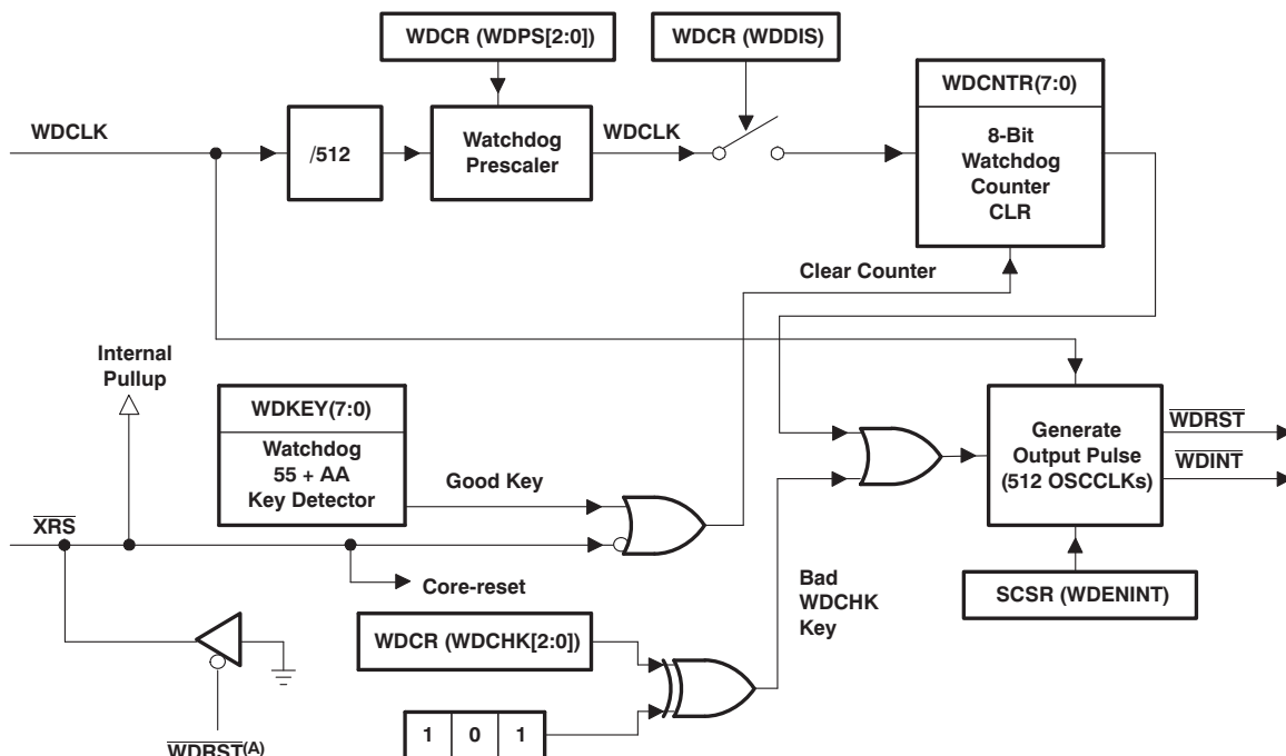
Figure 3-13. CPU-watchdog Module
