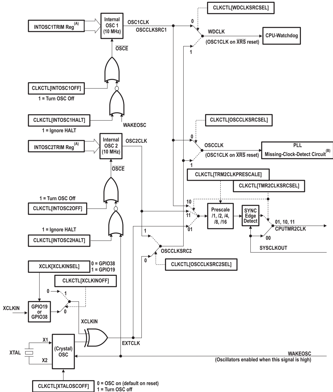
Figure 3-9. Clock Tree
