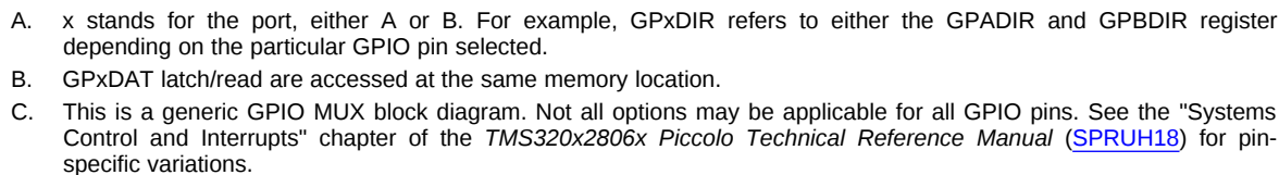
Figure 6-54. GPIO Multiplexing
