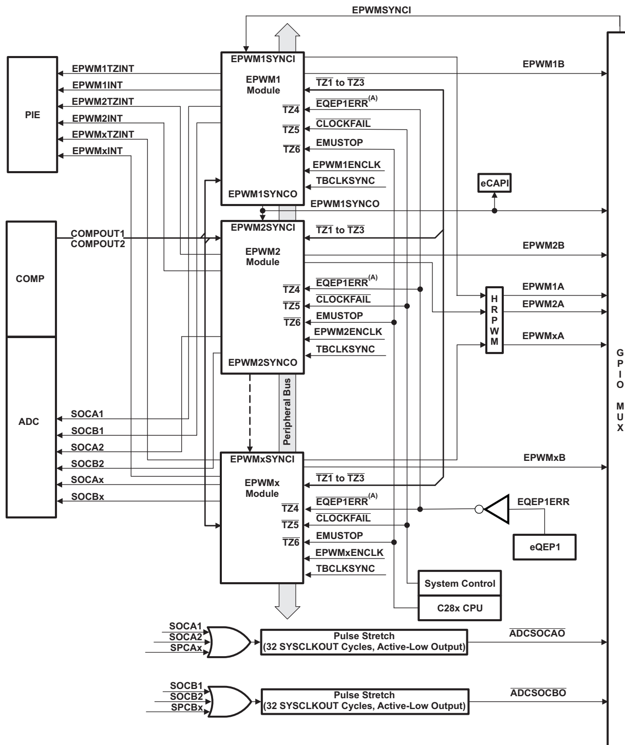
Figure 6-47. ePWM
