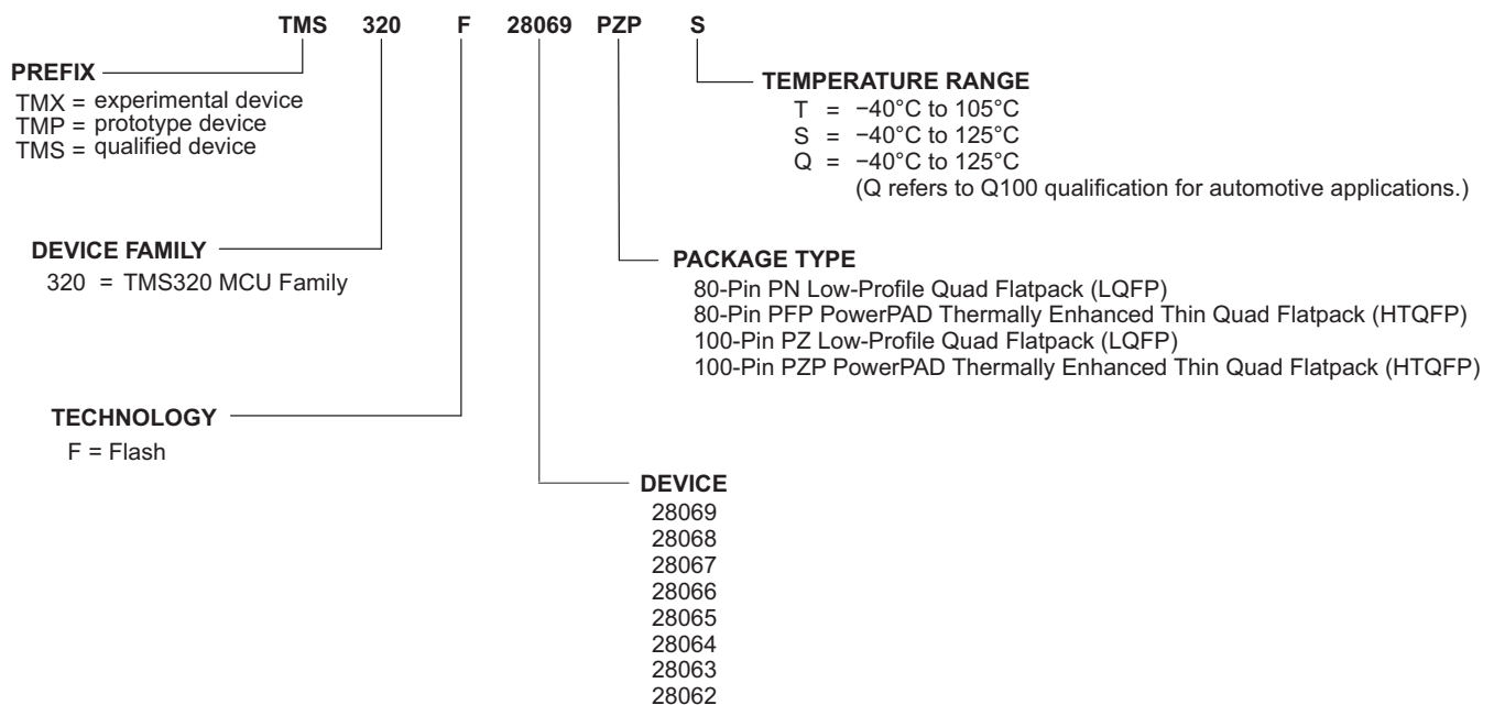
Figure 7-1. Device Nomenclature
