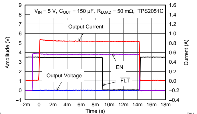
Figure 24. TPS2051C Enable into Short
