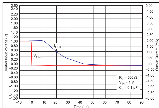
Figure 48. t_{OFF} Response
