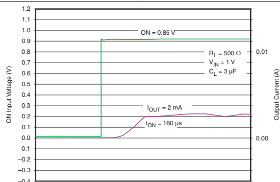
Figure 21. t_{ON} Response
