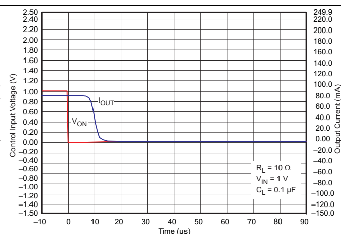
Figure 49. t_{OFF} Response
