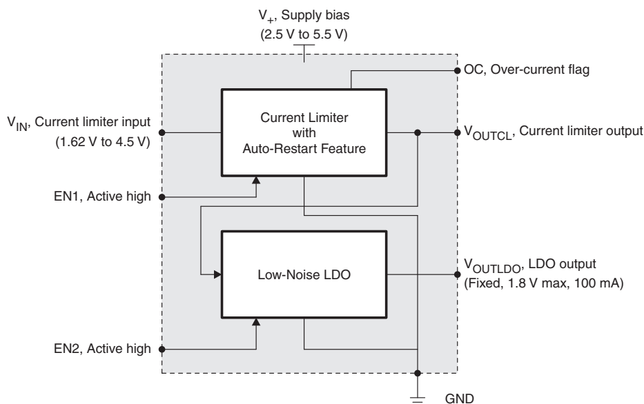
Figure 41. Simplified Block Diagram
