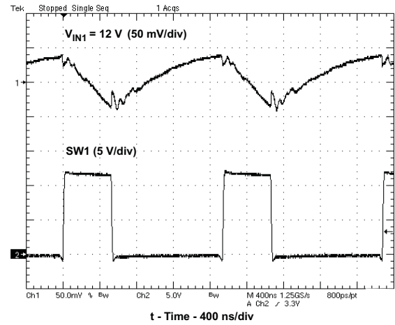
Figure 22. \text{VIN1} Input Voltage Ripple ( I_{O1}=2\text{A} )
