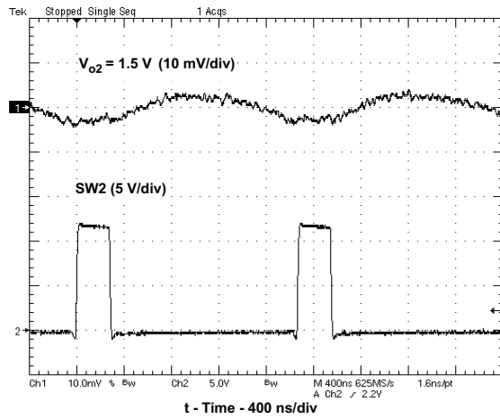
Figure 21. \text{VO2}=1.5\text{V} , Ripple Voltage ( I_{O2}=2\text{A} )
