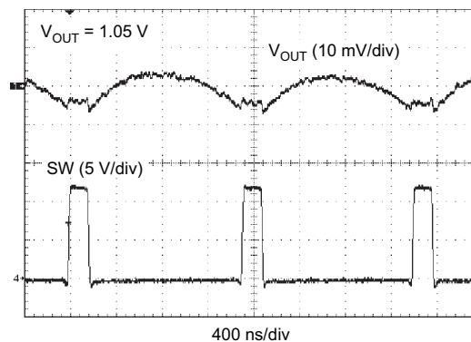
Figure 12. VOLTAGE RIPPLE AT OUTPUT ( I_0 = 3\text{ A} )
