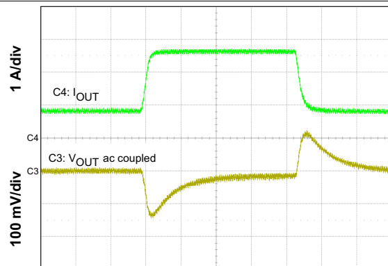
Time = 100 \mu\text{s}/\text{div} Figure 37. Load Transient
