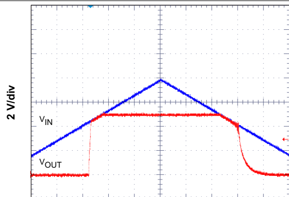
I_{OUT} = 100 \text{ mA} Time = 40 \mu\text{s}/\text{div} EN Floating
