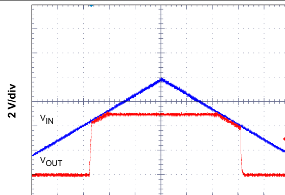
I_{OUT} = 1 \text{ A} Time = 40 \mu\text{s}/\text{div} EN Floating
