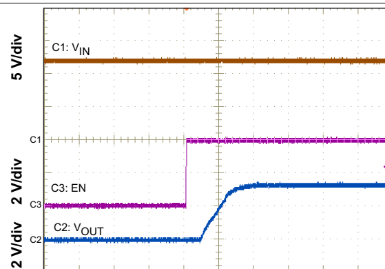
Time = 2 ms/div Figure 40. Start-up With EN
