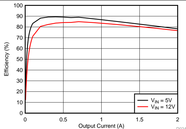
Figure 21. TPS562209 Efficiency
