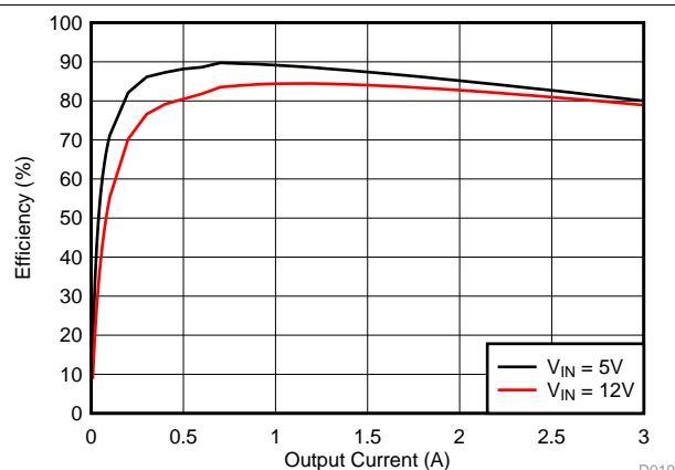
Figure 34. TPS563209 Efficiency
