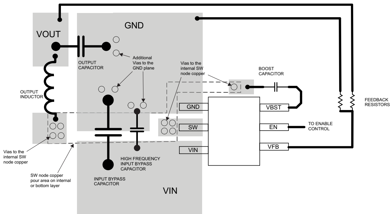
Figure 50. Typical Layout
