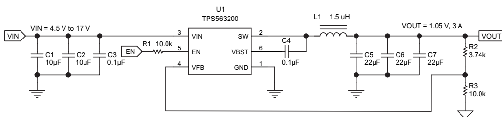
Figure 35. TPS563200 1.05V/3A Reference Design
