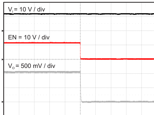
Figure 34. TPS562200 Shut Down Relative to EN
