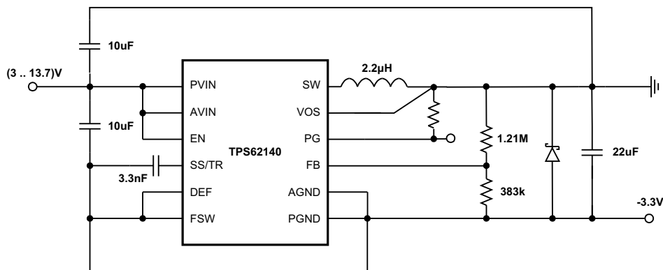
Figure 50. -3.3V Inverting Power Supply
