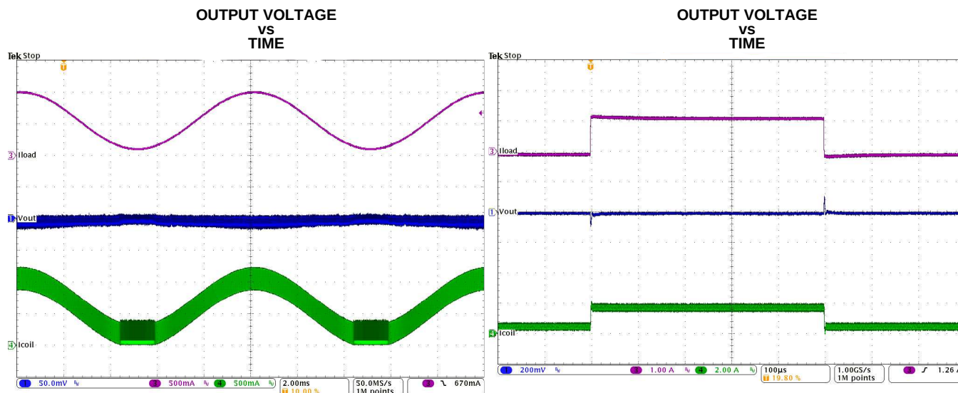
Figure 29. PWM-PSM-Transition ( V_{IN}=12\text{ V} , V_{OUT}=3.3\text{ V} With 50 mV/div)
