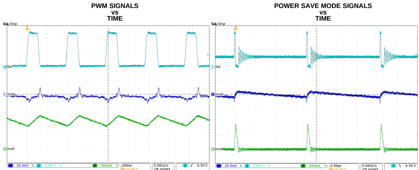
Figure 35. Typical Operation in PWM Mode (IOUT = 1 A)
