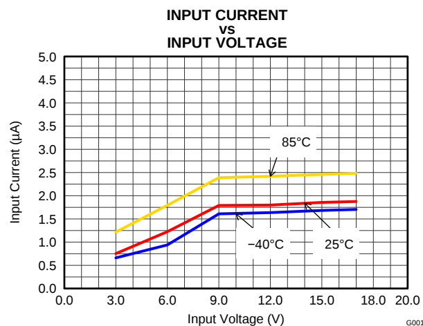
Figure 22. Shutdown Current
