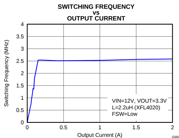
Figure 20. Switching Frequency
