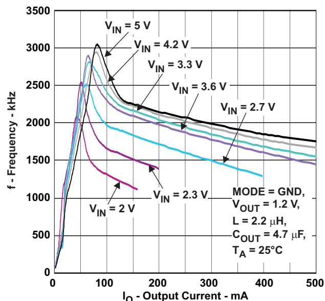
Figure 23. Switching Frequency vs Output Current, 1.2V Output Voltage MODE = GND
