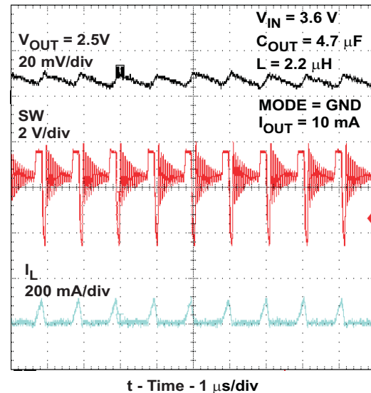
Figure 36. PFM Mode Operation I_{OUT} = 10\text{ mA}
