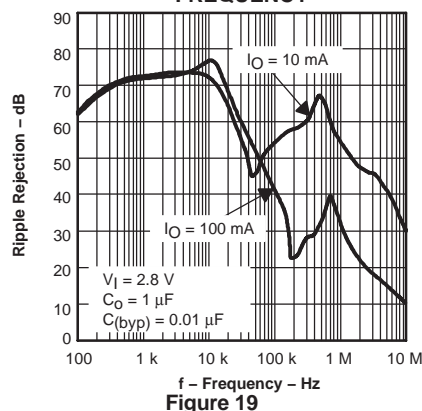
TPS79133 RIPPLE REJECTION VS FREQUENCY
