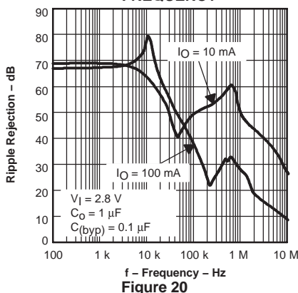
TPS79133 RIPPLE REJECTION VS FREQUENCY
