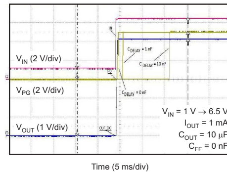
Figure 13. Power-Good Delay
