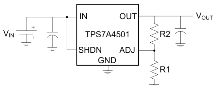
Figure 30. Adjustable Operation
