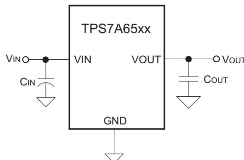
Figure 2. Application Schematic
