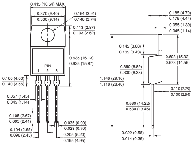
TO-220AB
