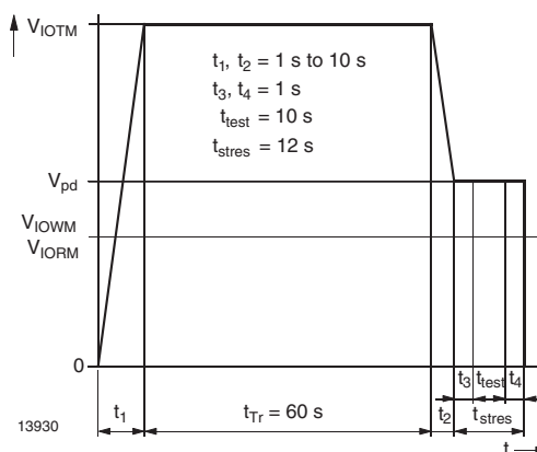
Fig. 5 - Test Pulse Diagram for Sample Test according to DIN EN 60747-5-5
