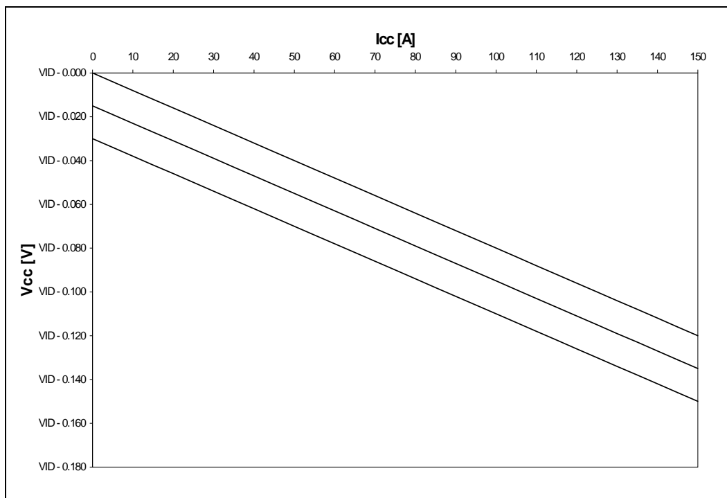
Figure 2-3. V CC Static and Transient Tolerance Loadlines 1,2,3,4
